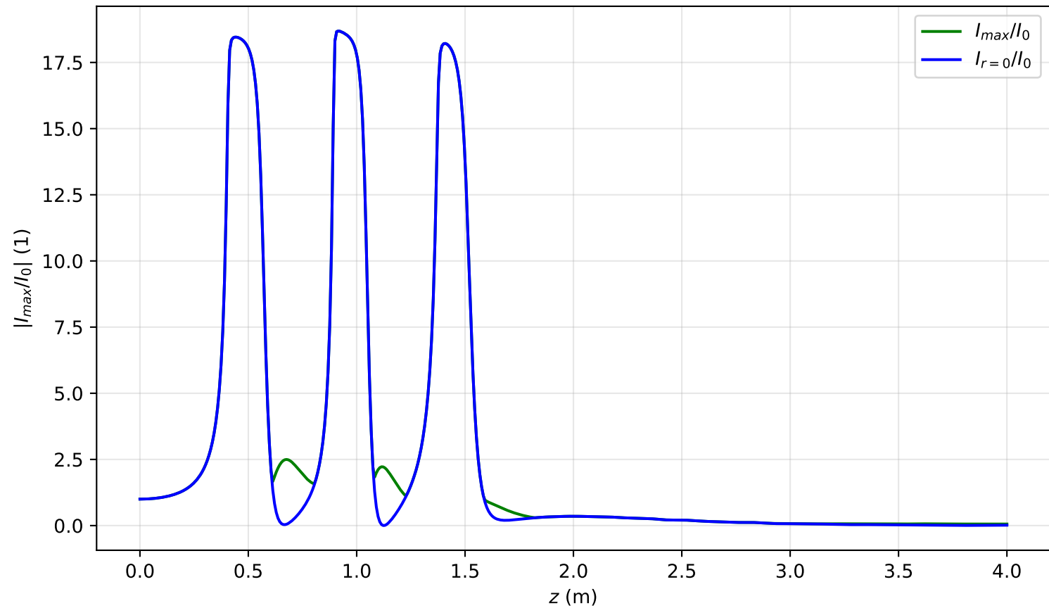
I_{max}(x=0, y=0, z)/I_0 , Pin=6.0Pcr, artificial time
